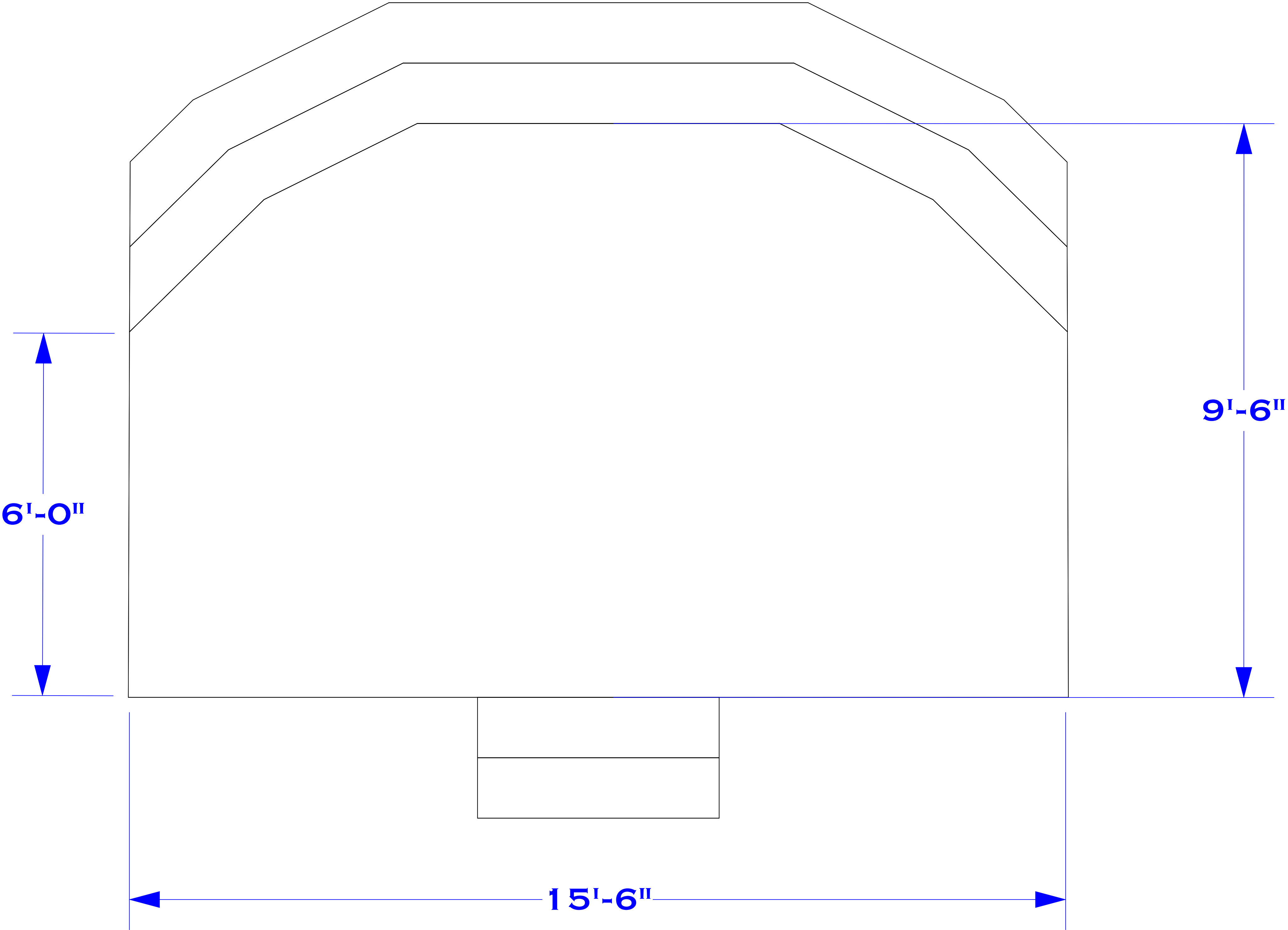
8 PLATFORM DIMENSIONS SCALE: 1" = 1'-0"
